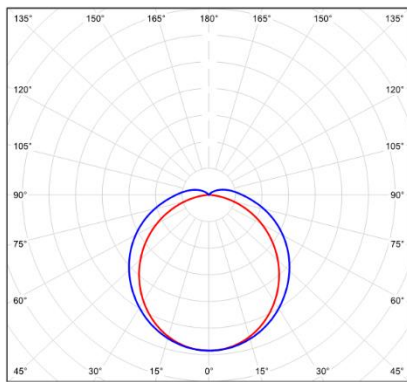
Polar Distribution
